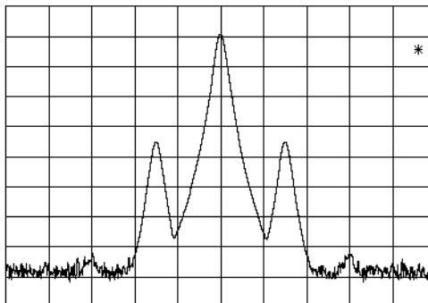
Figure 6-22 Using Time Gating to View Signal 1 (spectrum view)
