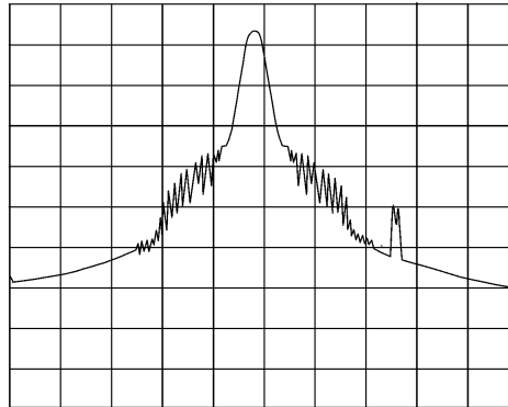
Figure 6-14 Time-Gated Spectrum of Radio 1
