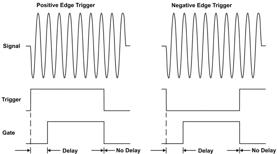
Figure 6-16 Edge Trigger Timing Relationships
