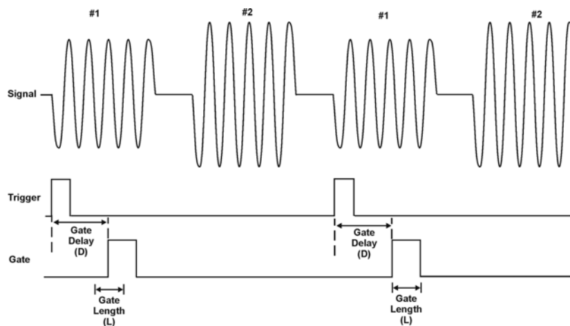
Figure 6-20 Timing Relationship of Signals During Gating
