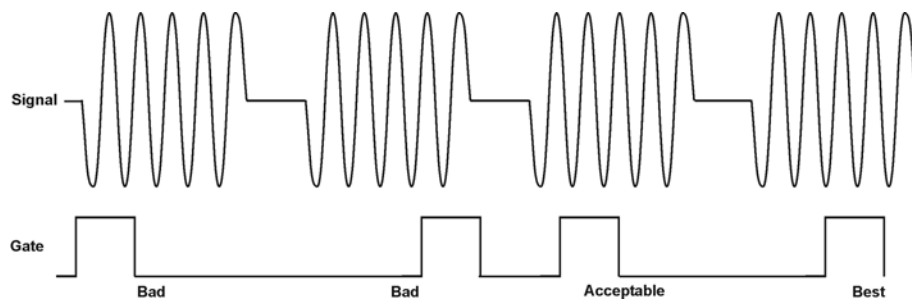
Figure 6-27 Best Position for Gate
