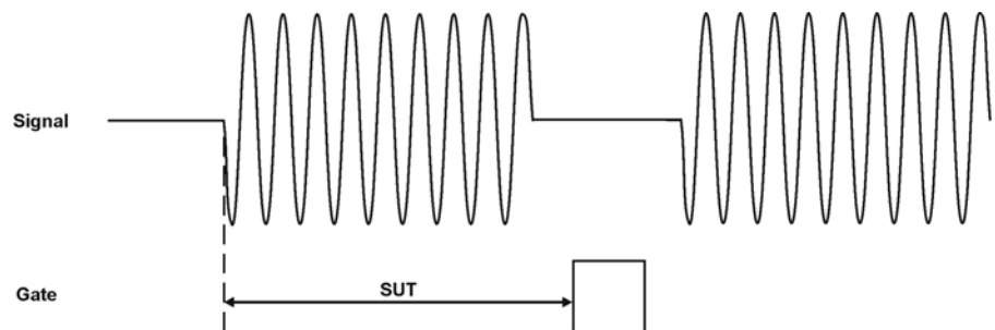
Figure 6-28 Setup Time for Interpulse Measurement
