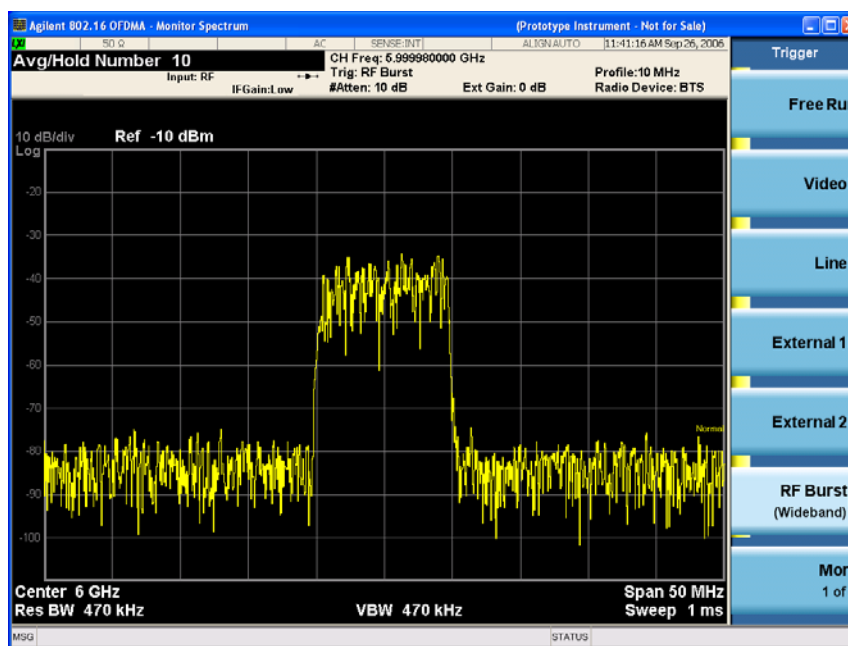
Figure 6-34 Monitor Spectrum Measurement Result w/ RF Burst Trigger
