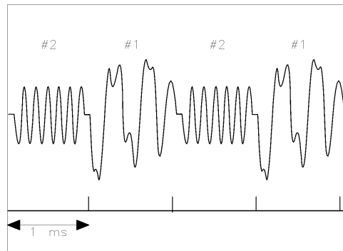
Figure 6-12 Simplified Digital Mobile-Radio Signal in Time Domain
