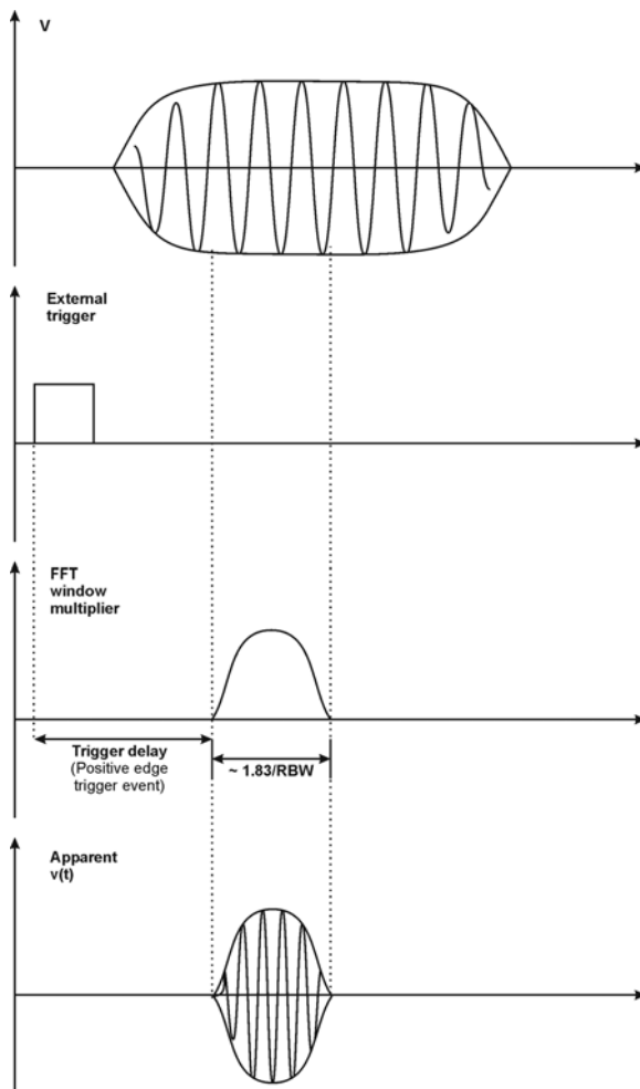
Figure 6-19 Gated FFT Timing Diagram
