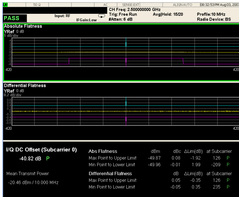
Figure 3-26 Modulation Analysis Measurement Result - Spectral Flatness View
