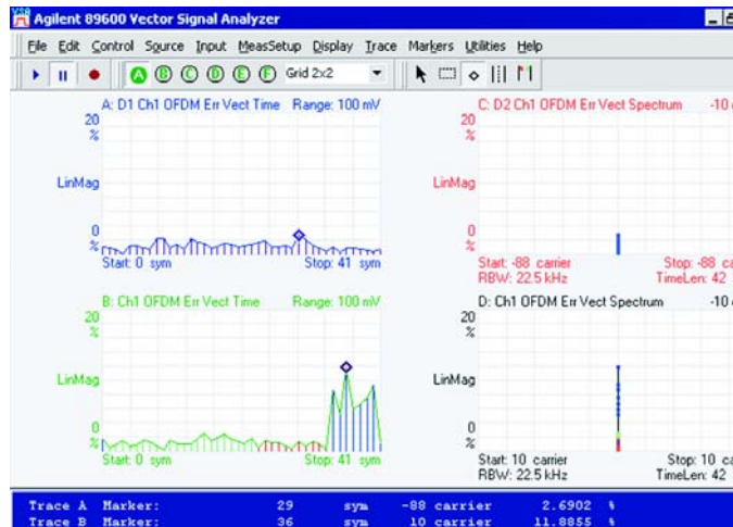
Figure 6-10 Error Vector Time and Error Vector Spectrum traces using a single WiMAX frequency subcarrier. The upper pair of traces shows the results for the pilot subcarrier at index = -88. The lower pair shows the results for a data subcarrier at index = 10 (example from Agilent 89600)
