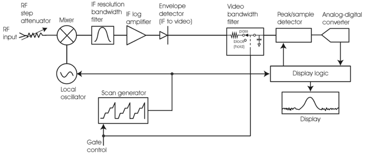
Figure 6-18 Gated LO Signal Analyzer Block Diagram
