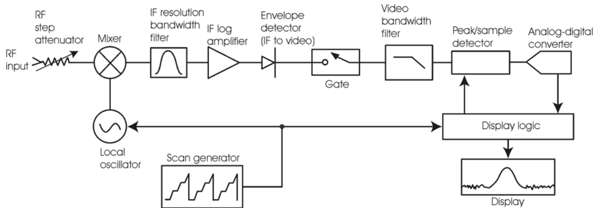
Figure 6-17 Gated Video Signal Analyzer Block Diagram
