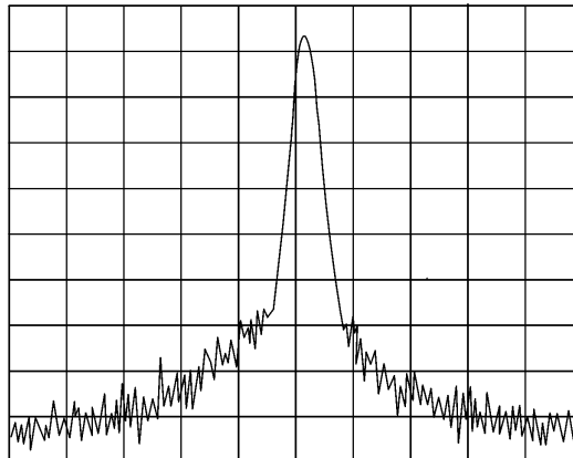
Figure 6-15 Time-Gated Spectrum of Radio 2
