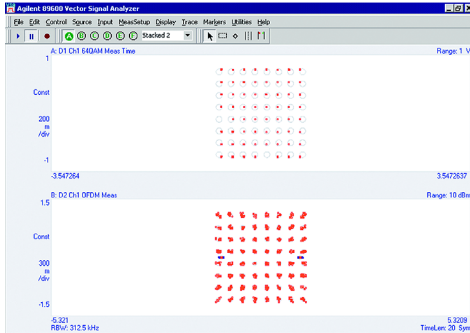
Figure 6-11 Constellation traces for single-carrier (upper trace) and OFDM (lower traces) modulated signals with IQ gain imbalance. Single-carrier Modulation OFDM Modulation pilot subcarriers (example from the Agilent 89600.)
