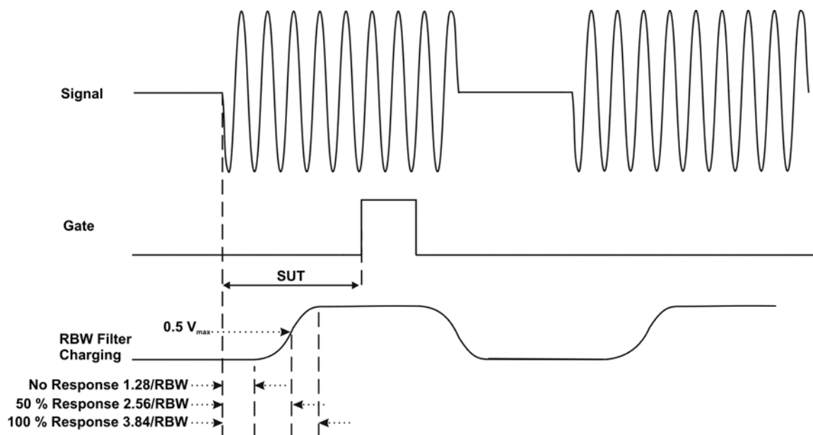
Figure 6-29 Resolution Bandwidth Filter Charge-Up Effects
